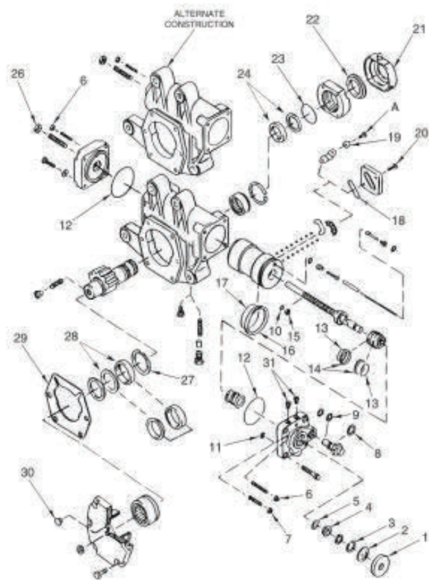
DIAGRAMA RK-914017
