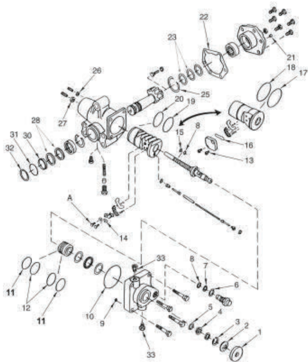
DIAGRAMA RK-914016
